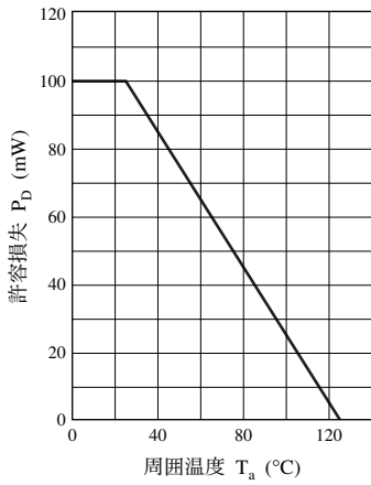
P_D - T_a
