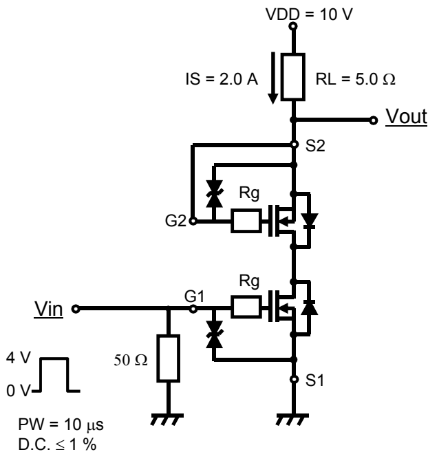
Note2: Measurement circuit
