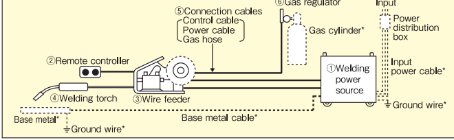
Standard Layout (non-remote type)
