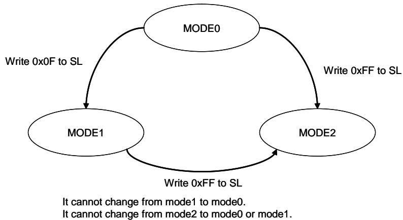
Figure 2-2 State Transition Diagram between System Lock Modes
