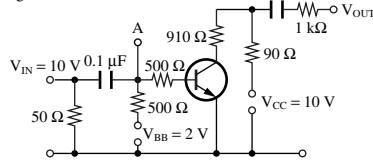
t_{stg} test circuit
