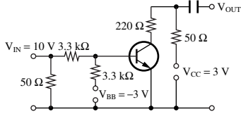
t_{on} , t_{off} test circuit
