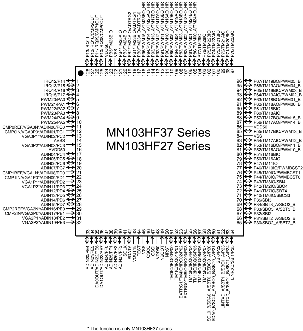
Figure:1.4.2 Pin Configuration of MN103HF37/27 Series
