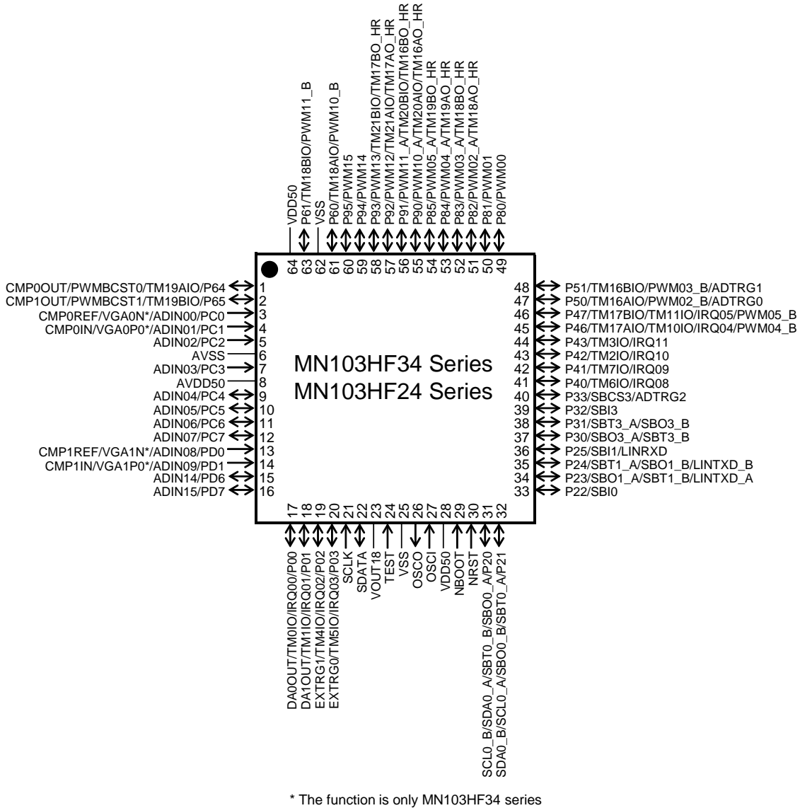
Figure:1.4.5 Pin Configuration of MN103HF34/24 Series
