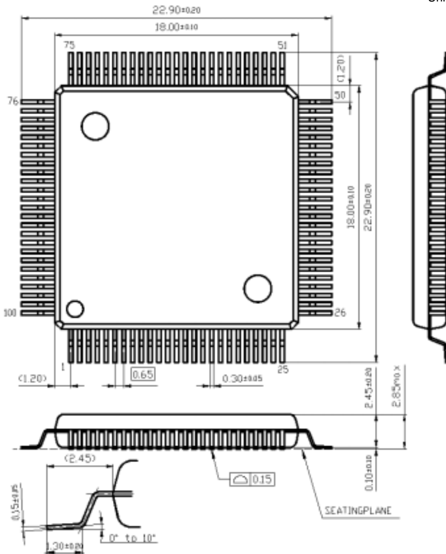
Figure:1.7.4 Package Dimension of 100 pin QFP
