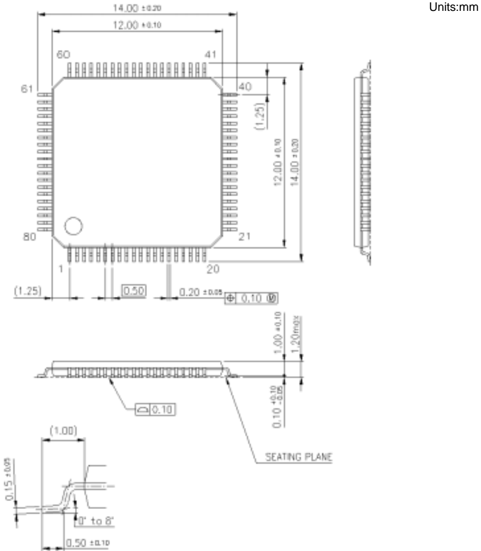
Figure:1.7.5 Package Dimension of 80 pin TQFP
