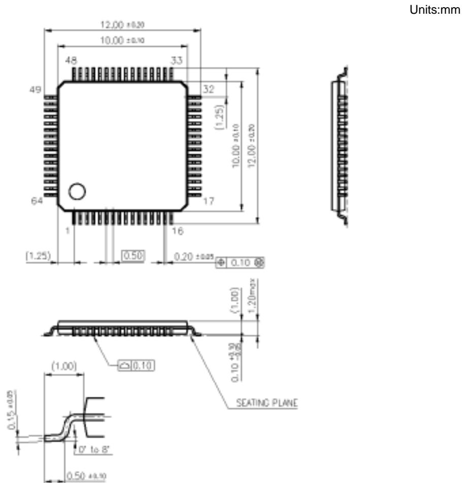
Figure:1.7.6 Package Dimension of 64 pin TQFP
