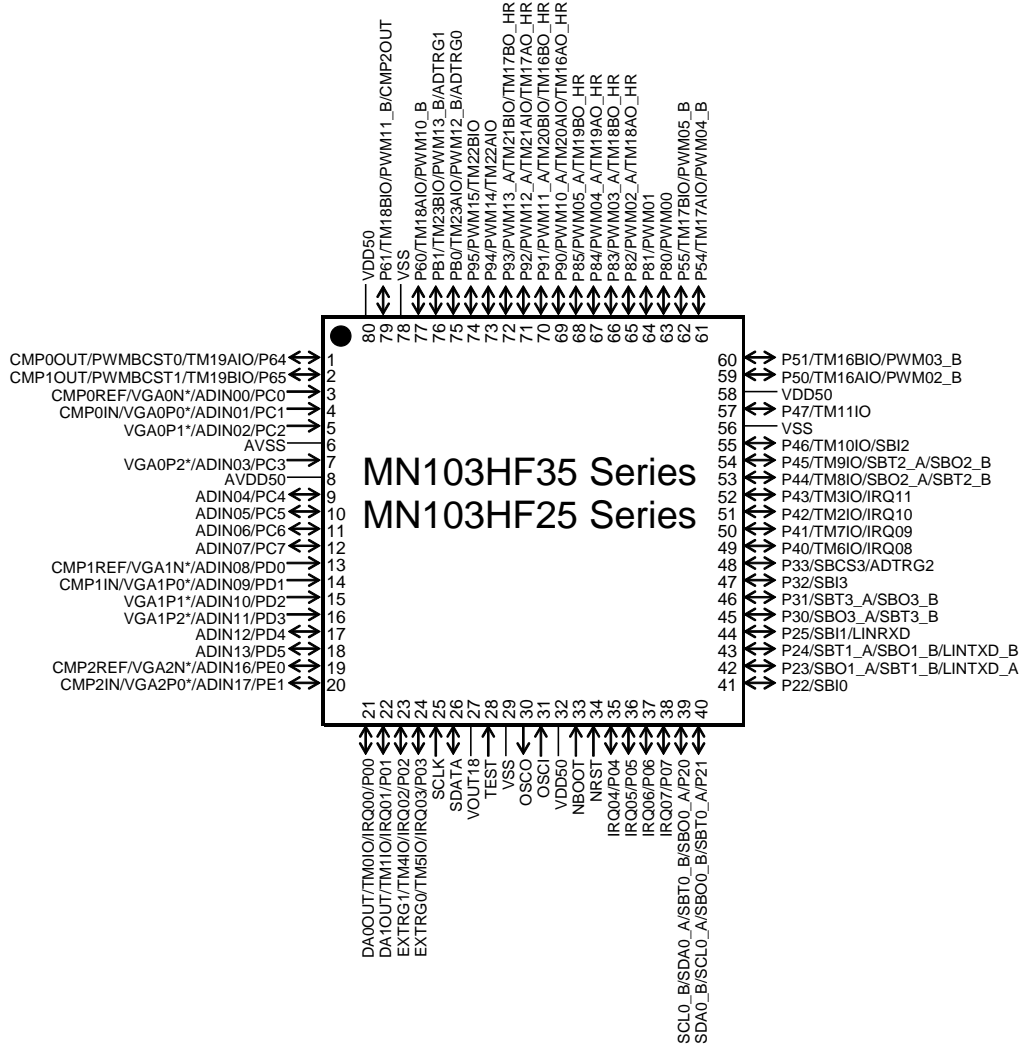
Figure:1.4.4 Pin Configuration of MN103HF35/25 Series
