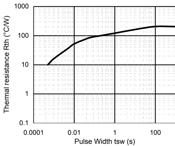
Rth -tsw
