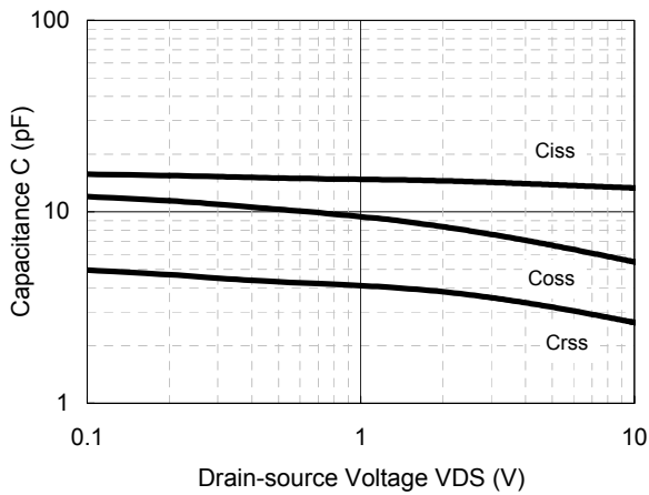
Capacitance - VDS
