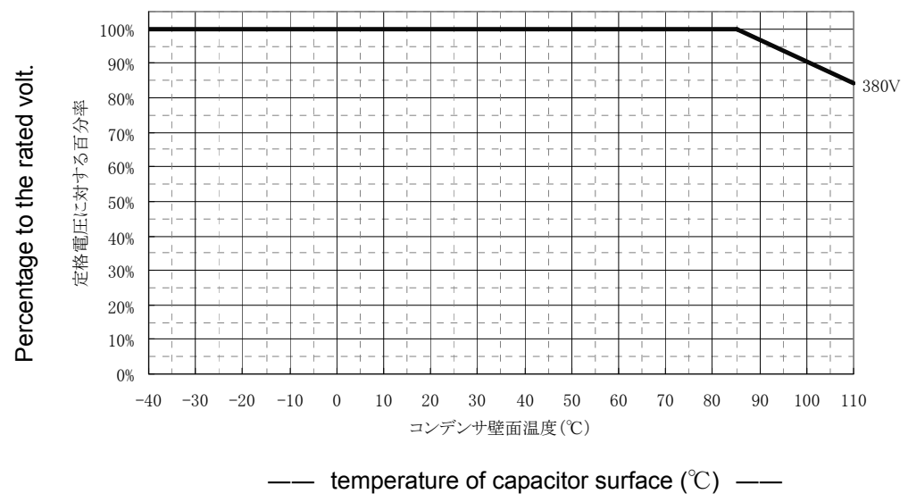
Fig.2 CURRENT DERATING VS. TEMPERATURE
