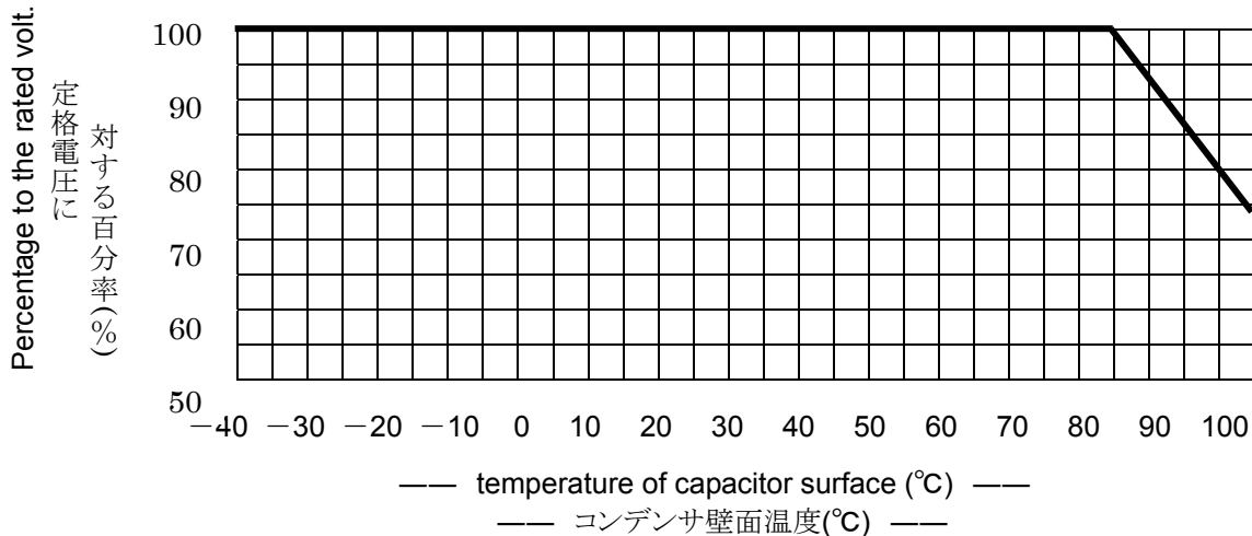
Fig.2 CURRENT DERATING VS. TEMPERATURE
