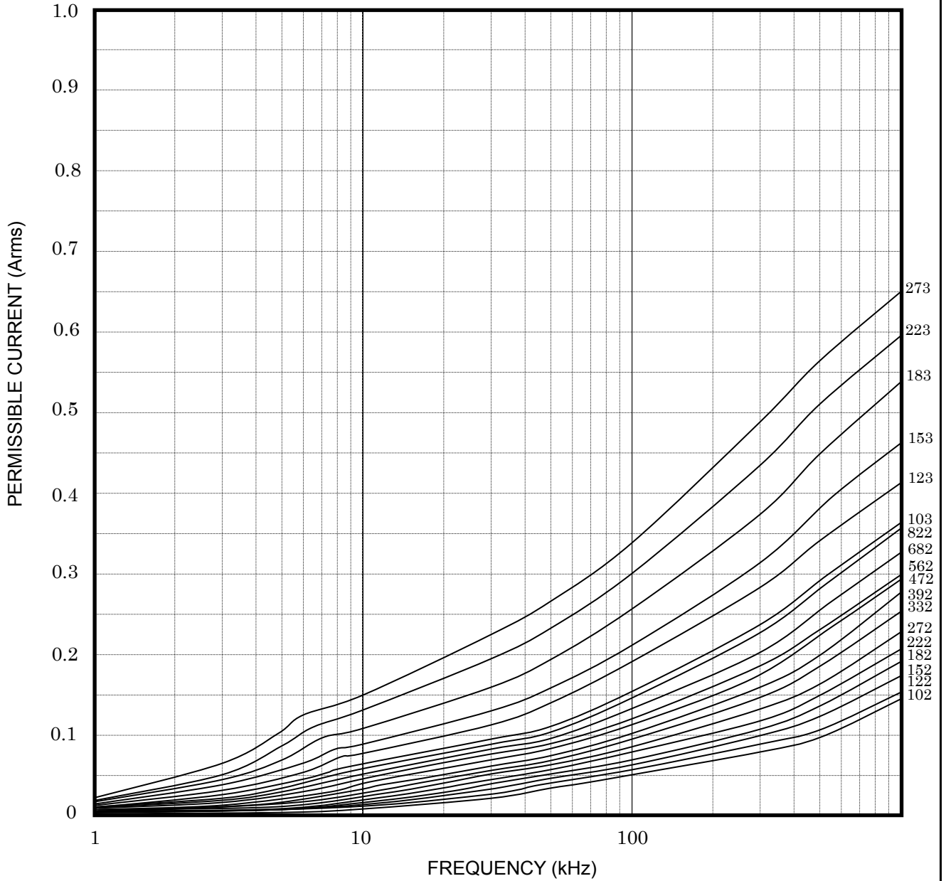
Fig.2-1 Permissible Current (0.0010 μF~0.027 μF) Measuring condition ●● Sine wave
