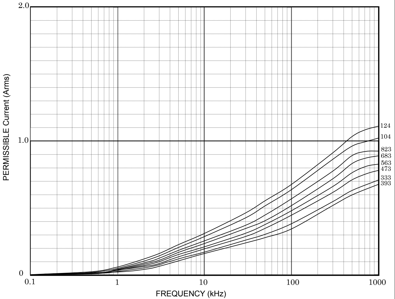
Fig.2-2 Permissible Current (0.033 \mu F~0.12 \mu F) Measuring condition ••• Sine wave
