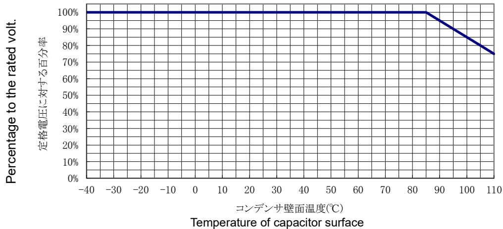
Fig.2 CURRENT DERATING VS. TEMPERATURE
