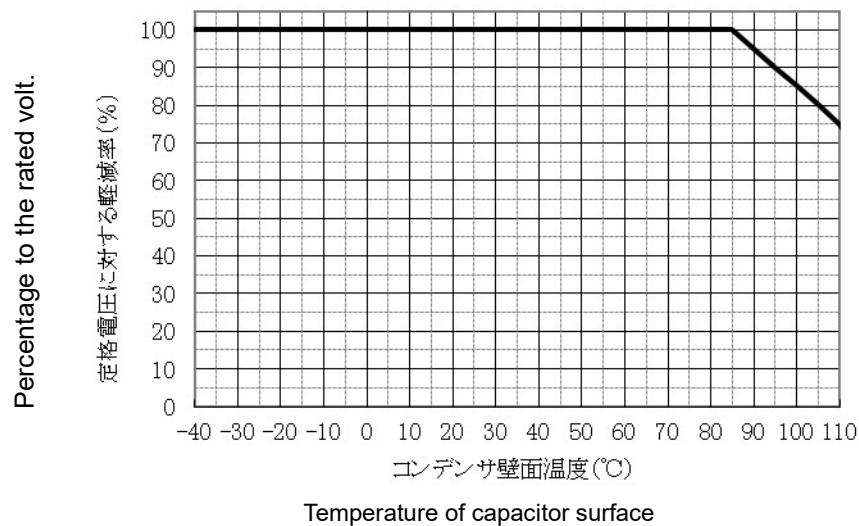
Fig.2 CURRENT DERATING VS. TEMPERATURE
