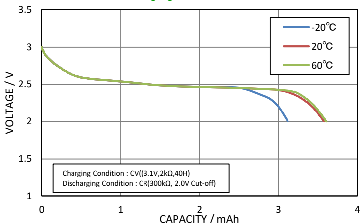
Discharging Characteristics
