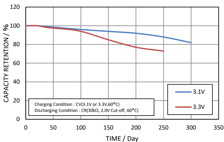
Continuous Charging Characteristics by High Temperature(60°C)
