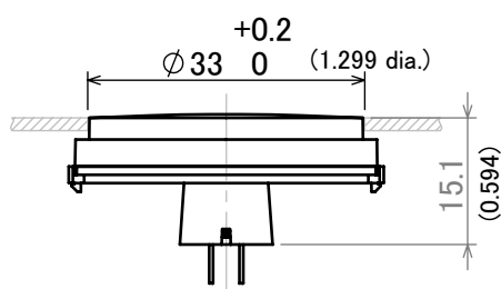
Recommended panel mouting hole dimensions
