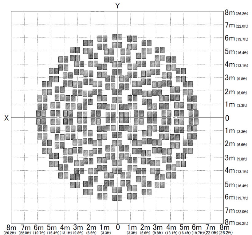
X-Y Cross Section (2.5m) (8.2ft)
