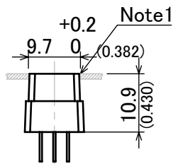
Recommended panel mouting hole dimensions
