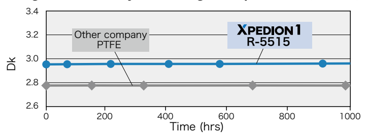
Long-term stability under high temperature (Dk, Df)
