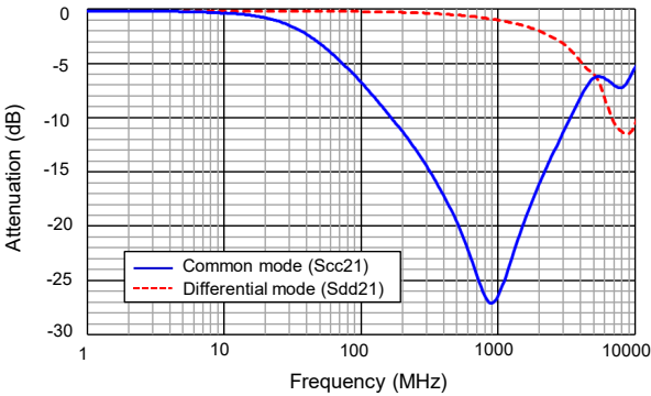
[ Attenuation characteristics ]
