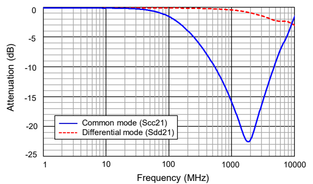
[ Attenuation characteristics ]
