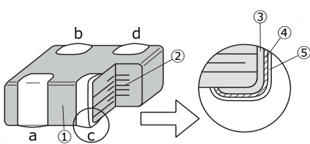
[构成]
