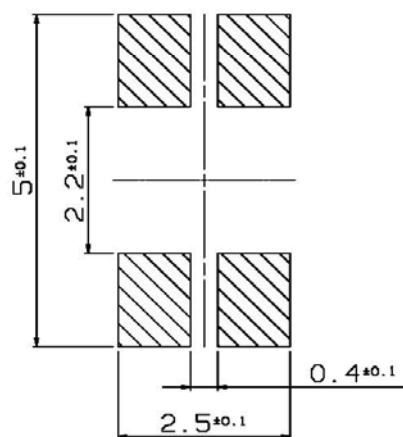
Land pattern plan
