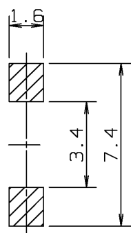
Land pattern plan
