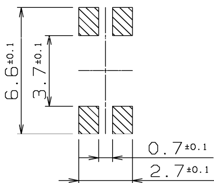
Land pattern plan
