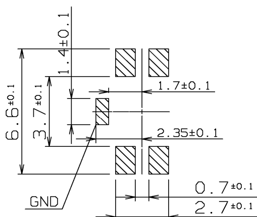
Land pattern plan
