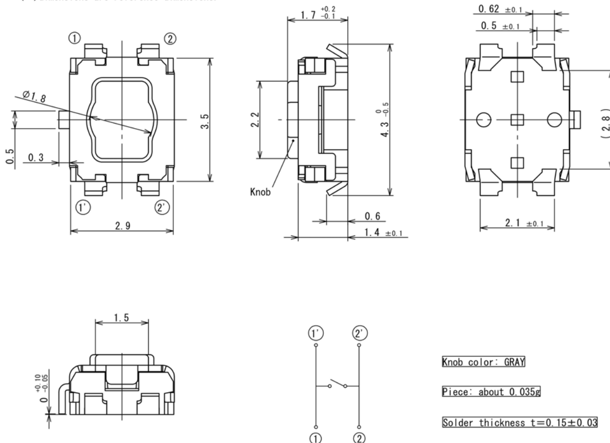
Circuit Diagram
