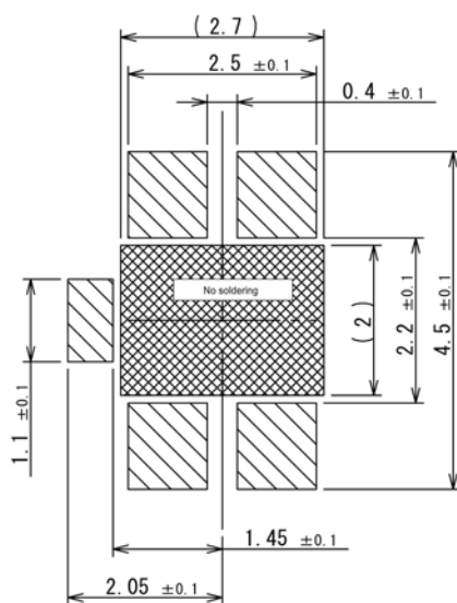
Land pattern plan
