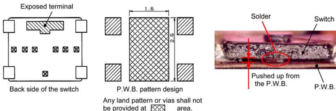
Fig2. P.W.B pattern design
