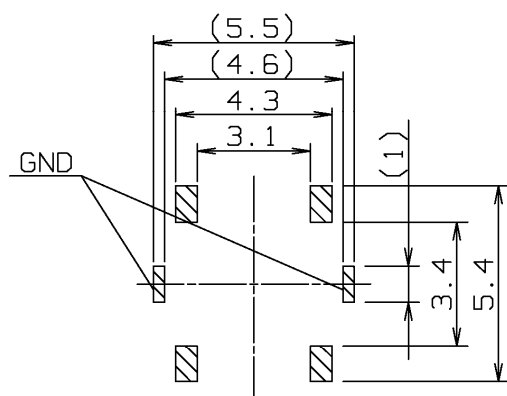
Land pattern plan
