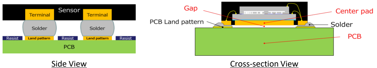
Figure 10-2 Solder Joint
