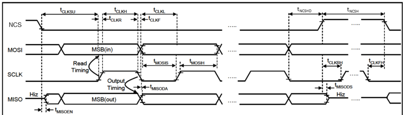
Figure 5-2 Timing Chart
