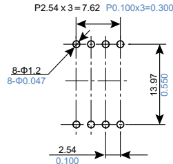
Recommended PC board pattern (TOP VIEW)
