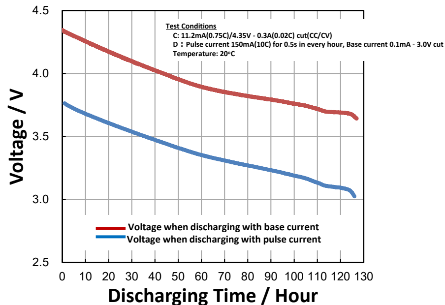
CG-320B Pulse discharging result with 150mA(10C)
