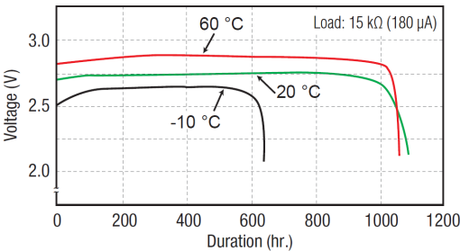
■ Discharge temperature characteristics (e.g. BR2032)
