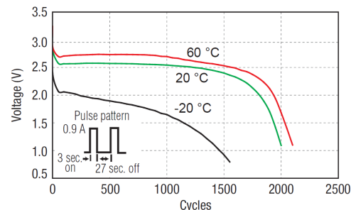
■ Discharge temperature characteristics(e.g. CR123A)
