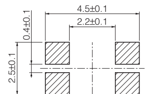
PWB land pattern for reference
