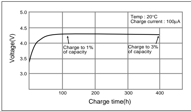
BR-2/3A (cylindrical type) charge test
